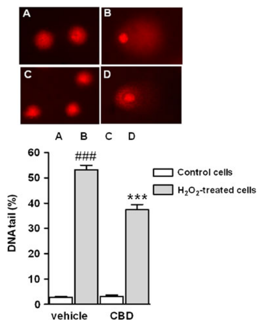
Fig. 7 Effect of cannabidiol (CBD, 10 μM for 24 h) on hydrogen peroxide (H 2 O 2 )-induced DNA damage evaluated by the comet assay. The DNA damage was induced in Caco-2 cells by 75 μM H 2 O 2 (b) and compared with PBS-treated (undamaged) cells (a). The effect of CBD was studied in presence (d) or absence (c) of H 2 O 2 . a–d Representative comets. Each bar represents the mean±SE mean of three independent experiments where at least 75 cells per gel in triplicate were scored. ### P <0.001 vs undamaged cells (a, PBS) and *** P <0.001 vs damaged cells (b, H 2 O 2 ). DNA damage, expressed as percentage of fluorescence in the comet tail (% DNA tail) was quantified using at least 75 cells per gel were scored and each sample was evaluated in triplicate ( n =3 independent experiments)
